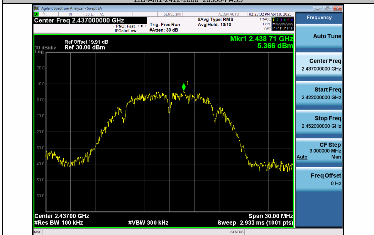
11B-Ant1-2437-0~Reference-PASS
