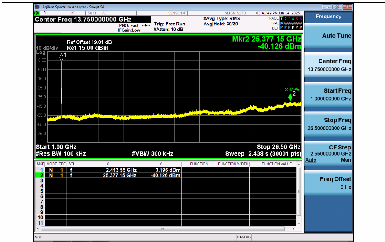
11N20SISO-Ant1-2412-1000-26500-PASS
