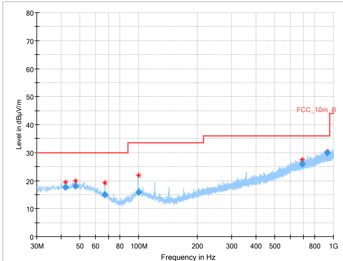
Plot 2: 30 MHz – 1 GHz, vertical and horizontal polarization, T Max UP Pro
