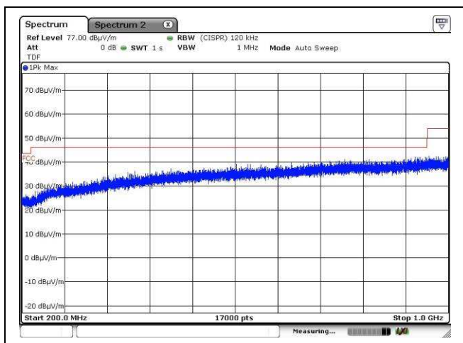
Charging mode, 200MHz – 1GHz, Horizontal
