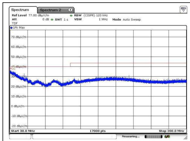
Charging mode, 30MHz – 200MHz, Vertical
