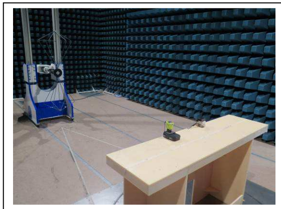
30MHz – 200MHz (Charging, front view)
