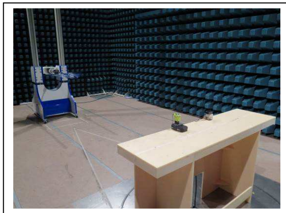
200MHz – 1GHz (Charging, front view)
