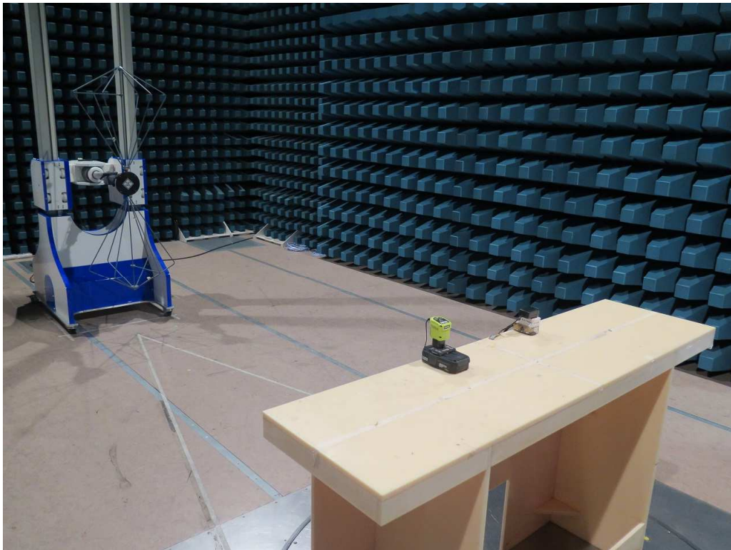
30MHz – 200MHz (Front view, charging)
