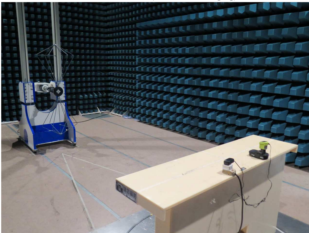
30MHz – 200MHz (Rear view, charging)
