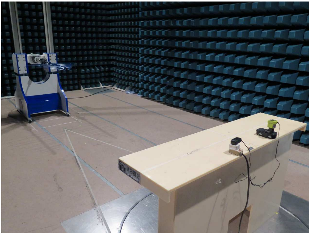
200MHz – 1GHz (Rear view, charging)
