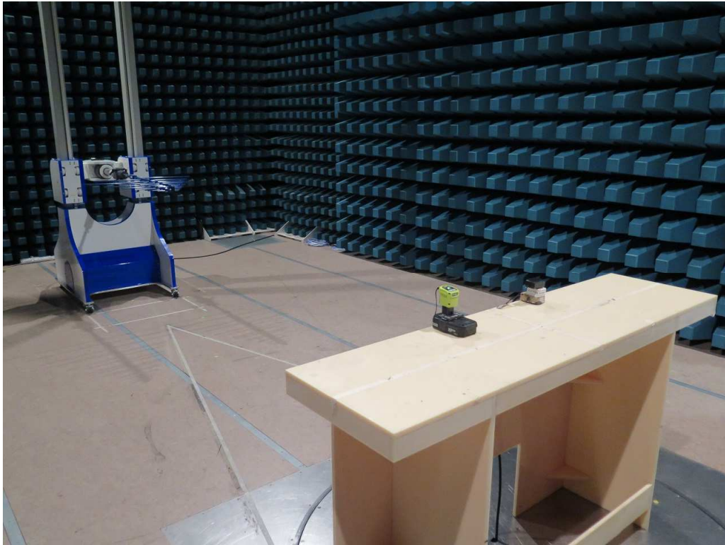
200MHz – 1GHz (Front view, charging)
