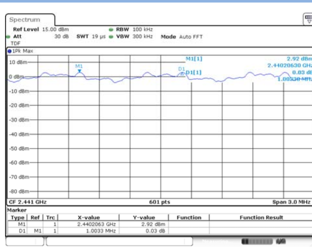
8-DPSK
