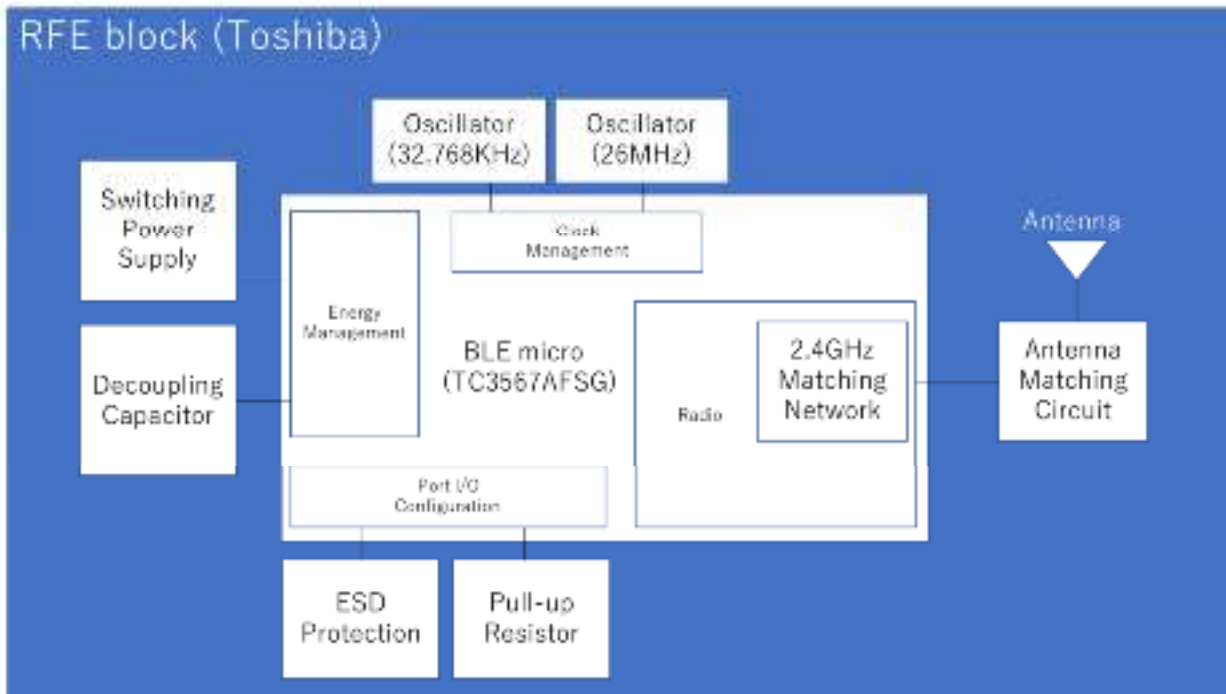
Figure 2: RFE Block of Toshiba BLE IC (current)
