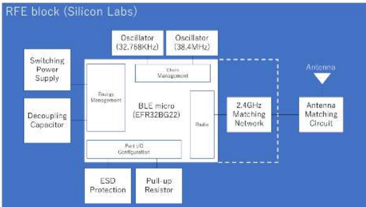
Figure 3: RFE Block of Silicon Labs BLE IC (proposed)
