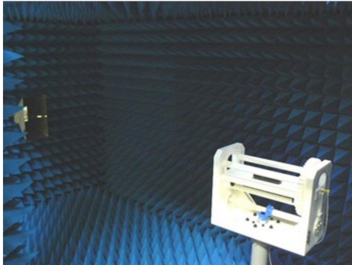
Figure 2 – Anechoic Chamber at PHC in Matsuyama
