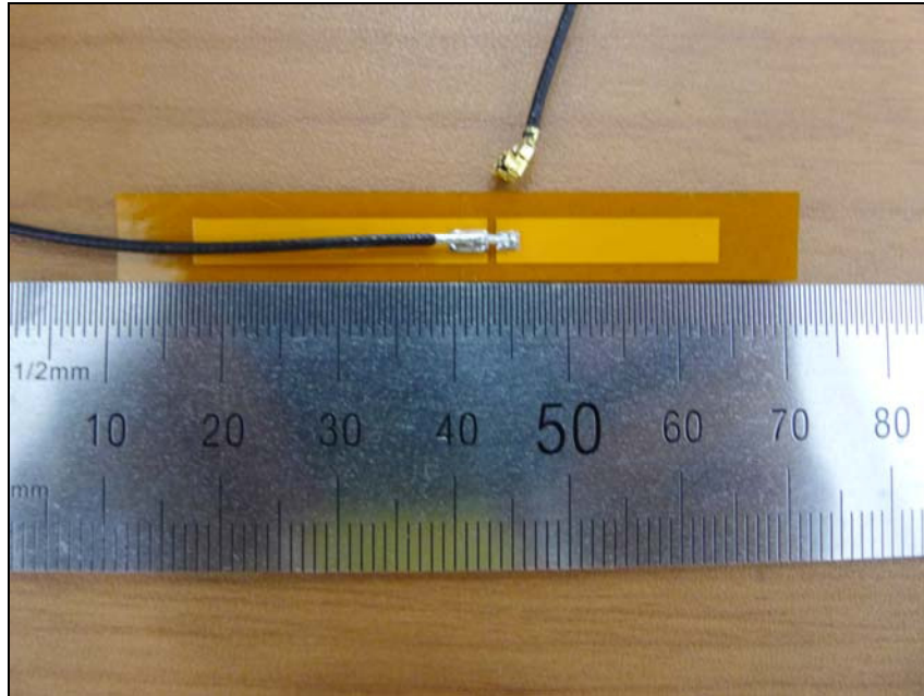
Antenna (FPCB type antenna)
