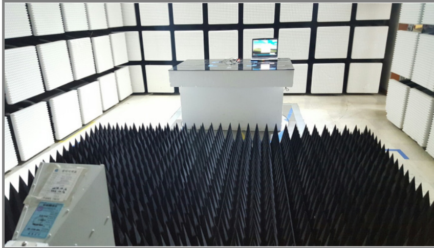
Photo of radiated spurious emission at above 1 000 MHz
