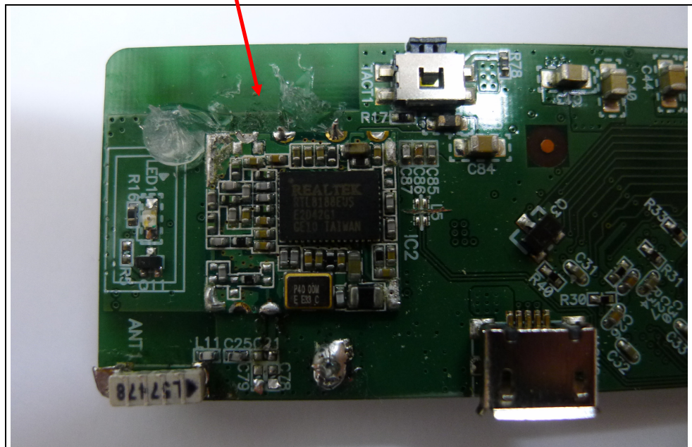
WLAN Module (removed shield case)
