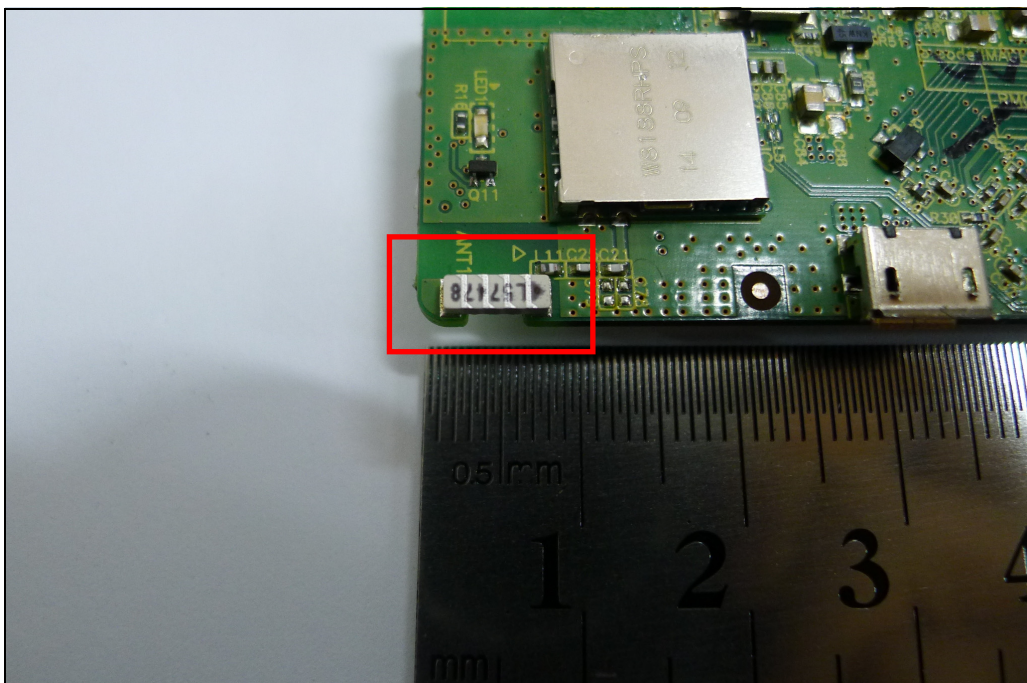
Antenna(WLAN)
