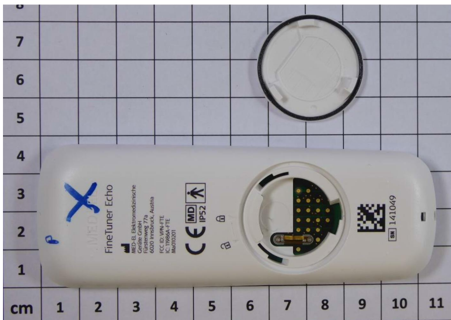
(EUT back view with open battery compartment)
