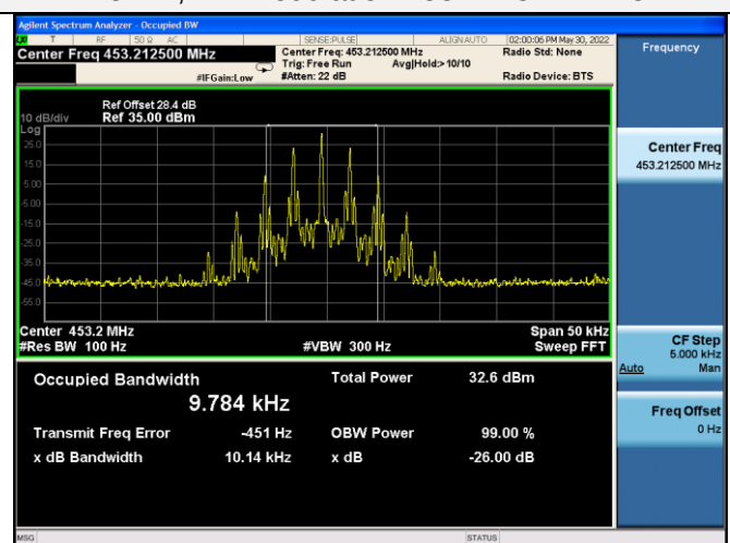
12.5kHz, FM Modulation:453.2125MHz-2.5W
