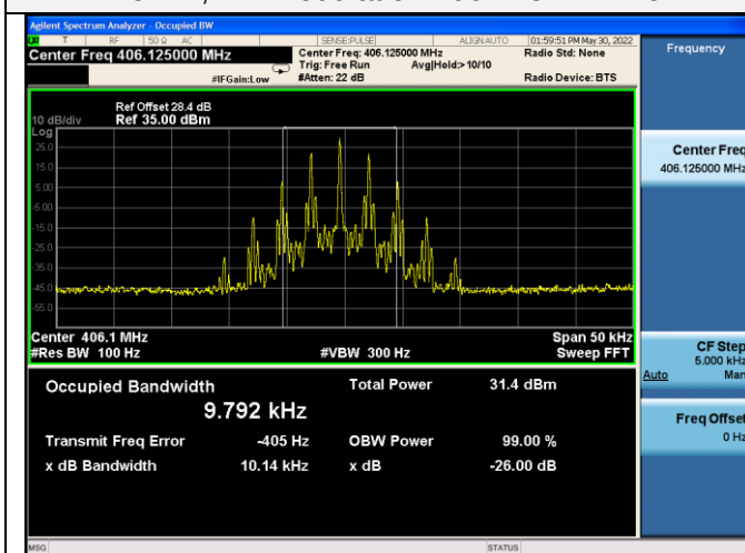
12.5kHz, FM Modulation:406.125MHz-2.5W
