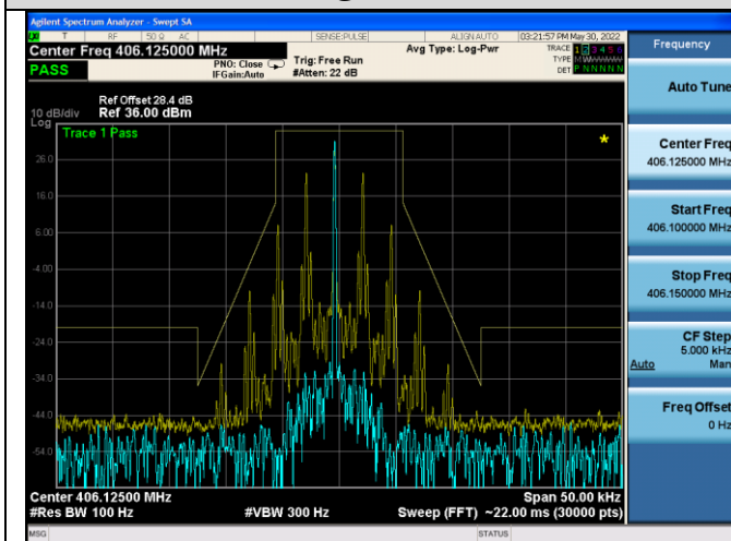
Emission Mask D@406.125MHz-2.5W-FM
