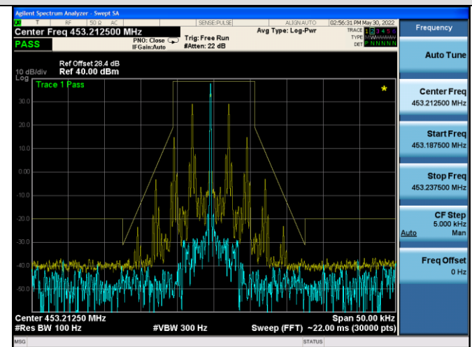
Emission Mask D@479.975MHz-7W-FM
