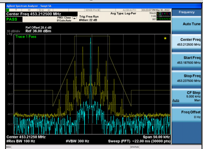
Emission Mask D@453.2125MHz-2.5W-FM
