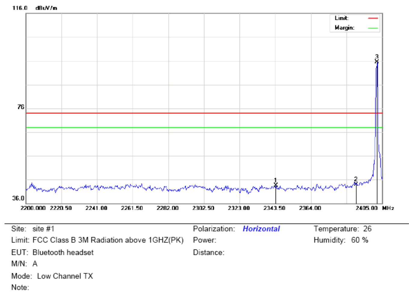
TEST PLOT OF BAND EDGE FOR LOW CHANNEL-Horizontal
