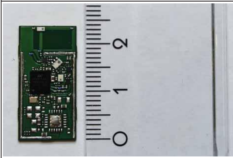
ENWF9408A2EF_top_nocase
