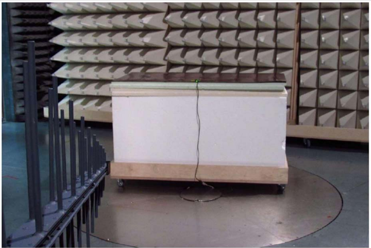
Radiated Setup - View D
