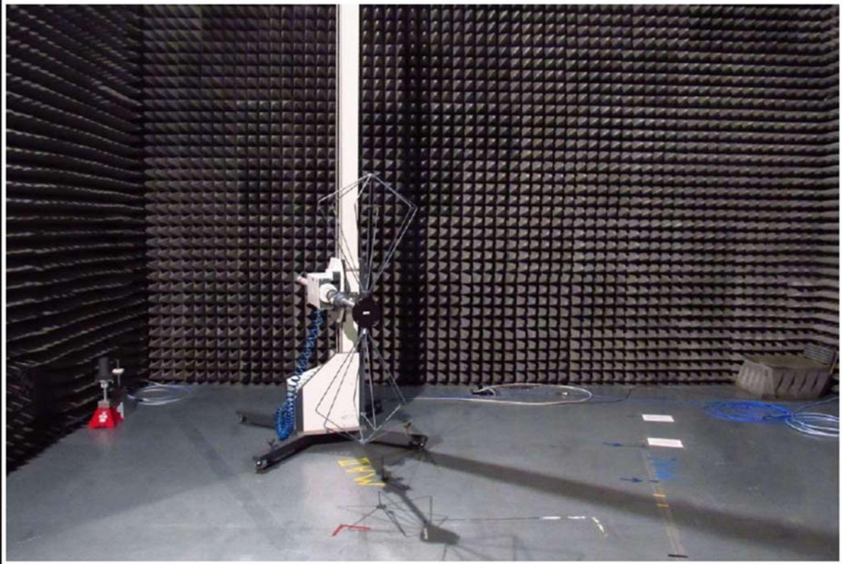
Radiated Setup - View C
