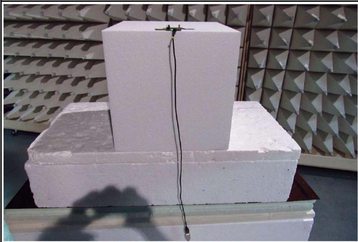
Radiated Setup - View F
