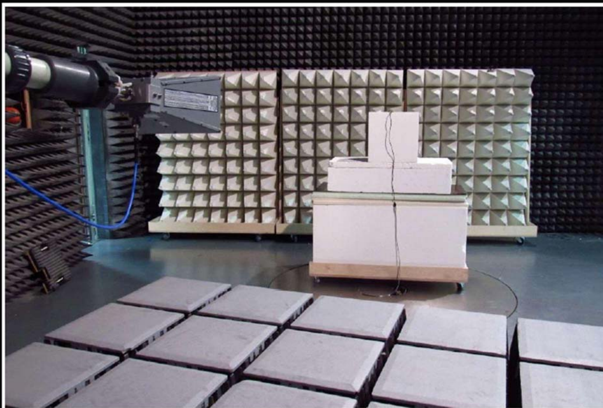
Radiated Setup - View G
