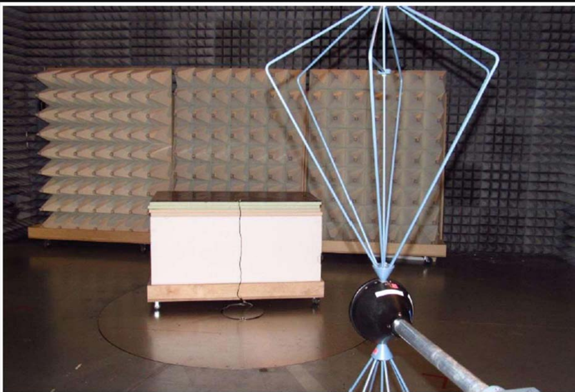
Radiated Setup - View B
