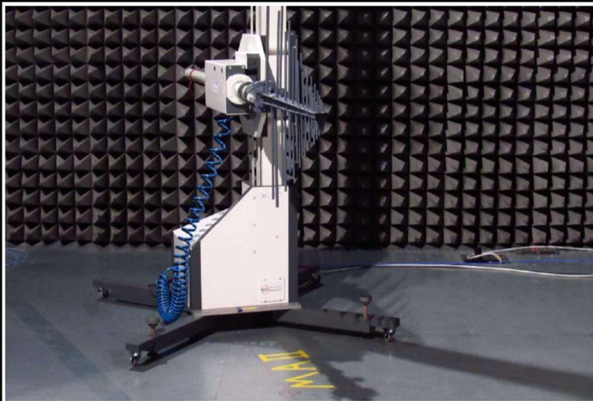
Radiated Setup - View E
