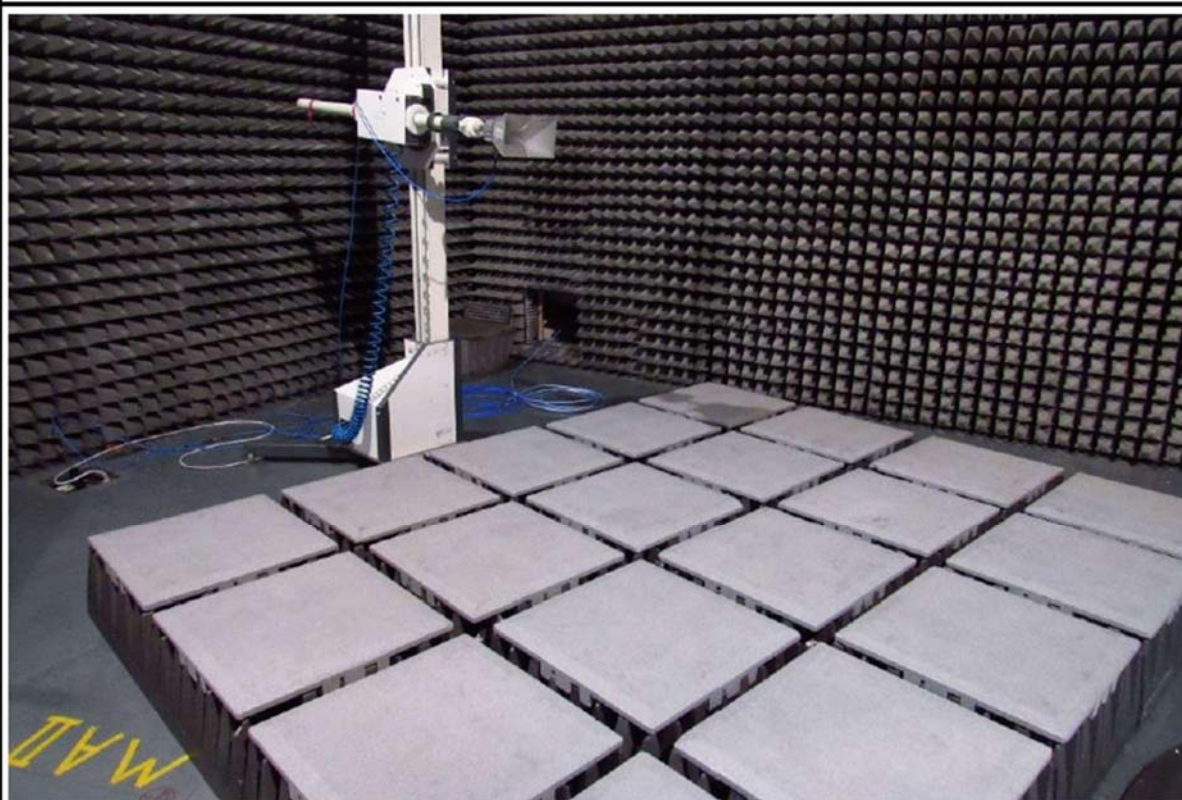
Radiated Setup - View H
