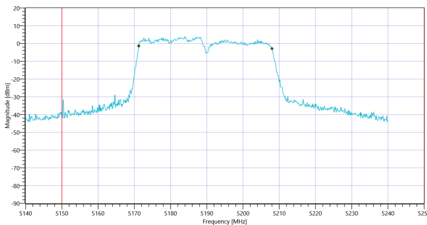
Plot_FCC Part 15.407 & ISED Bandwidths ~ WLAN5Gx n-HT40 mode U-NII-1_18082021_105900.png
