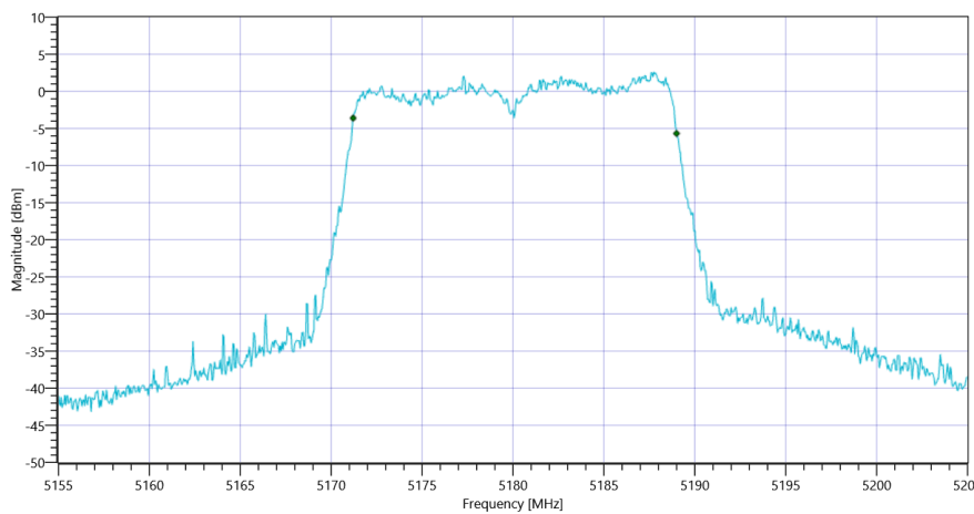
Plot_FCC Part 15.407 & ISM Bandwidths ~ WLAN5Gx n-HT20 mode U-NII-1 99PCT_18082021_100600.png
