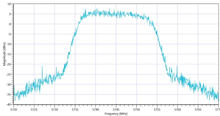
Plot_Common 5Gx-6Gx Peak OP 3MHz-3MHz ~ WLAN5Gx a mode U-NII-3_18082021_092427.png
