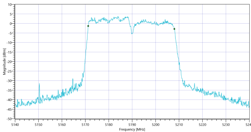
Plot_FCC Part 15.407 & ISED Bandwidths ~ WLAN5Gx n-HT40 mode U-NII-1 99PCT_18082021_105853.png
