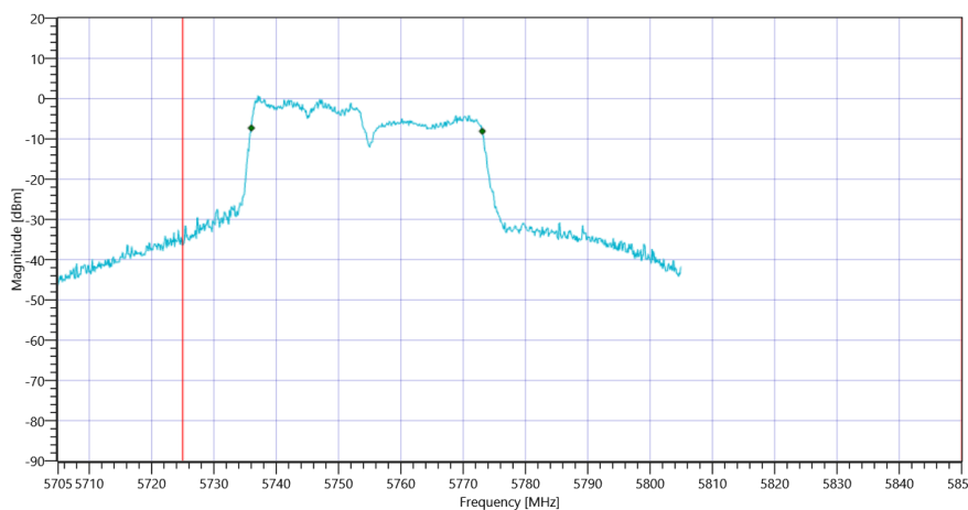
Plot_FCC Part 15.407 & ISM Bandwidths ~ WLAN5Gx n-HT40 mode U-NII-3_18082021_111434.png
