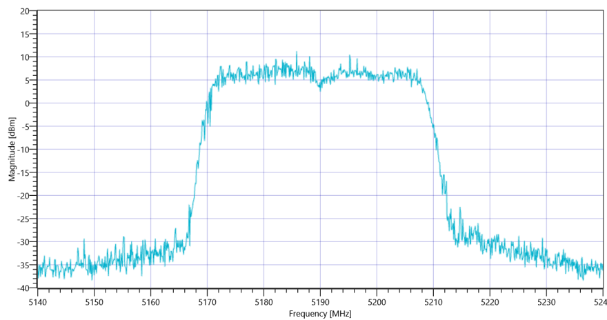
Plot_Common 5Gx-6Gx Peak OP 3MHz-3MHz ~ WLAN5Gx n-HT40 mode U-NII-1_18082021_105446.png
