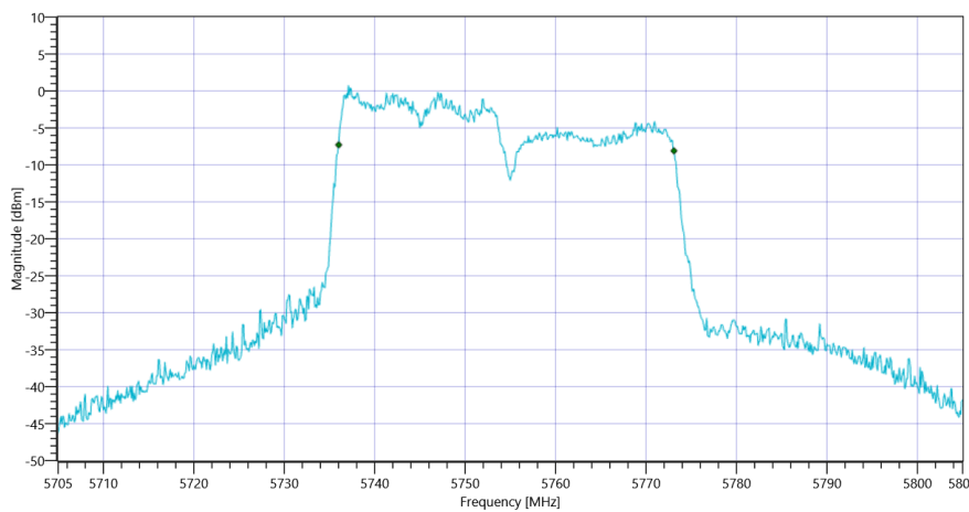
Plot_FCC Part 15.407 & ISM Bandwidths ~ WLAN5Gx n-HT40 mode U-NII-3 99PCT_18082021_111427.png
