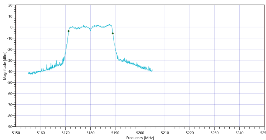
Plot_FCC Part 15.407 & ISM Bandwidths ~ WLAN5Gx n-HT20 mode U-NII-1_18082021_100607.png
