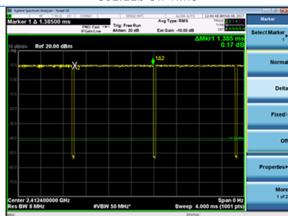
802.11g On-Time
