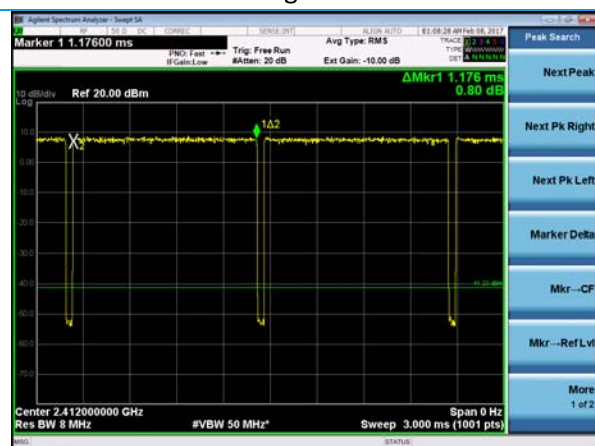
802.11n On-Time
