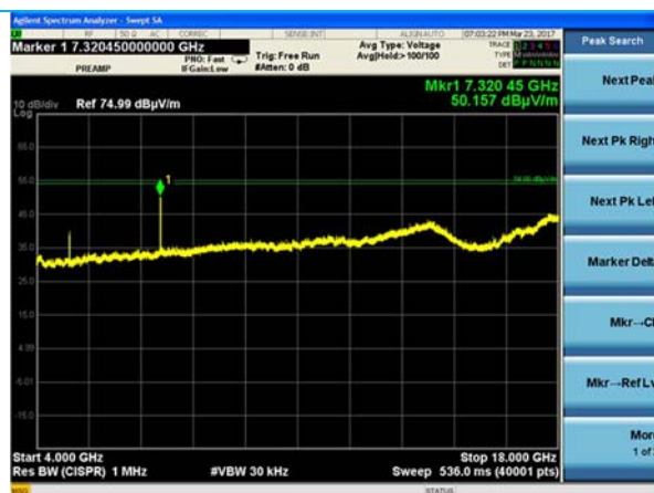
Mid Channel – 4-18 GHz – Reduced VBW
