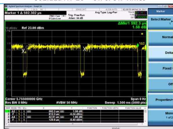
802.11a HT-40 – On & Off-Times
