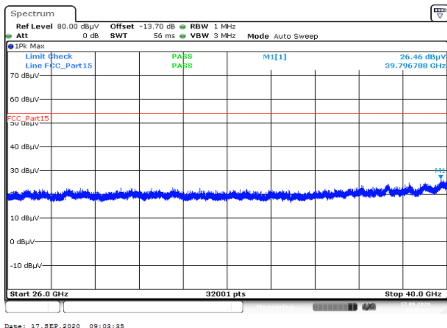
Plot 6: 26 GHz to 40 GHz; vertical & horizontal polarization; U-NII-2A; highest channel
