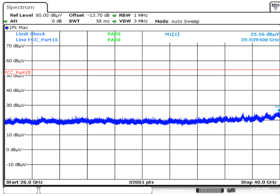
Plot 18: 26 GHz to 40 GHz; vertical & horizontal polarization; U-NII-3; lowest channel
