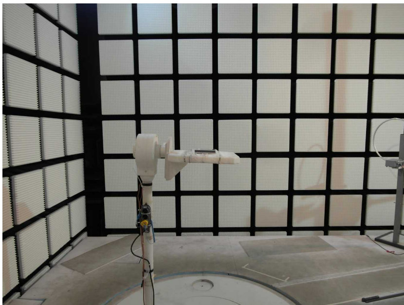
Photo 6 RSE > 1GHz
