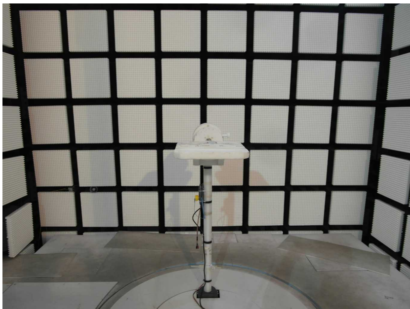
Photo 4 RSE > 1GHz
