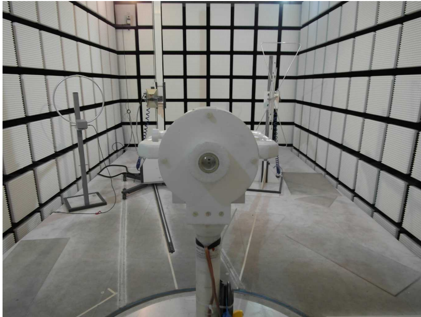
Photo 5 RSE > 1GHz
