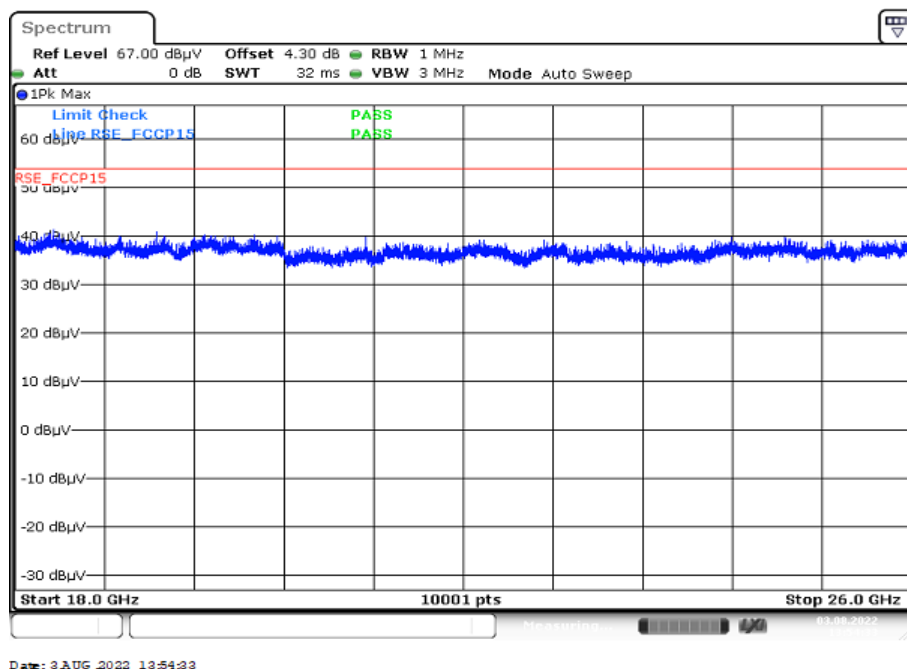
Plot 4: All channels, 18 GHz to 26 GHz, vertical & horizontal polarization
