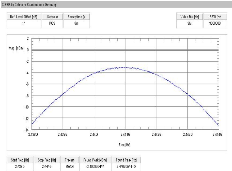
Plot 5: middle channel – 2441 MHz, Pi / DQPSK modulation
