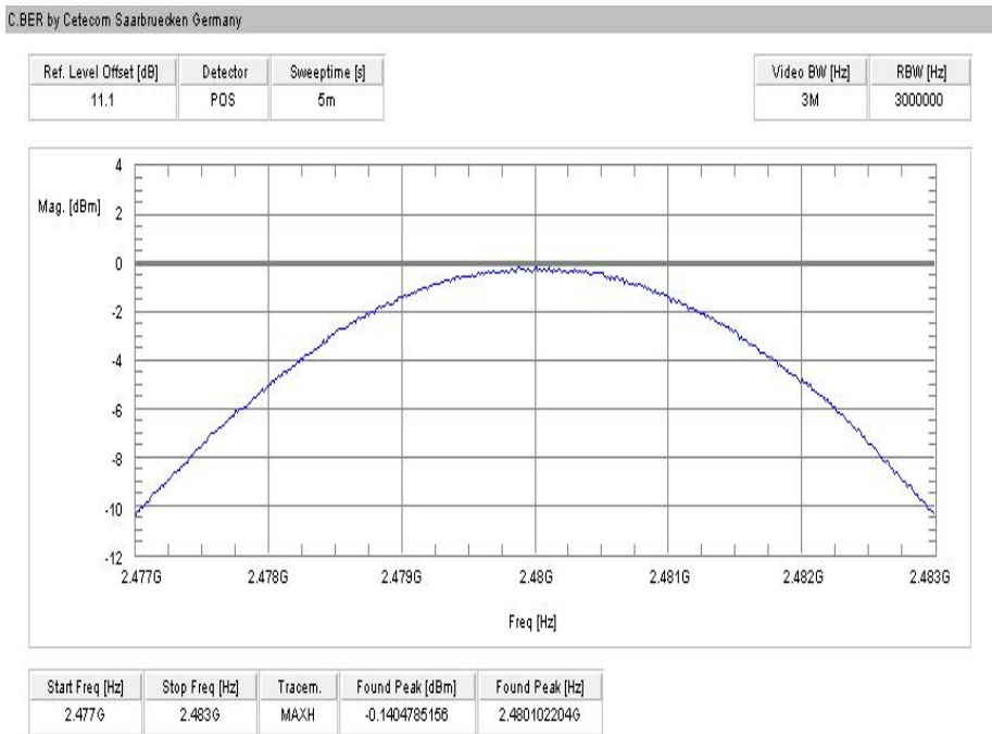
Plot 6: highest channel – 2480 MHz, Pi / DQPSK modulation
