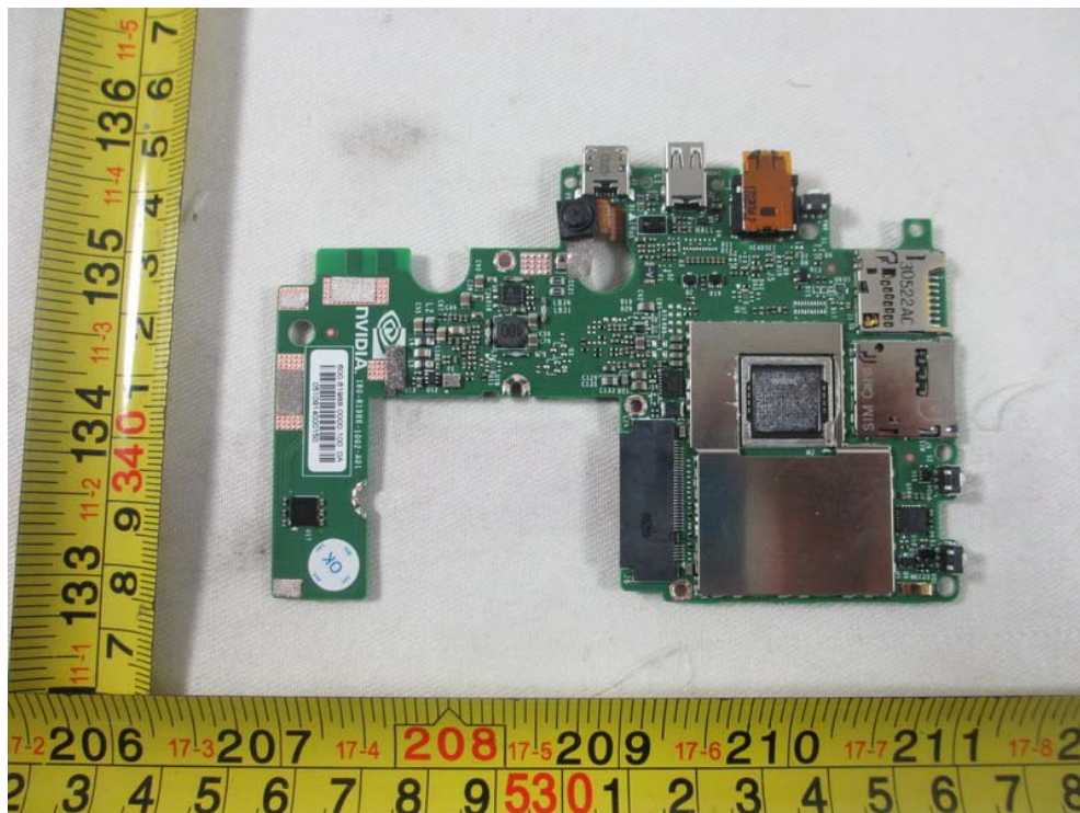
BT, WIFI Board
