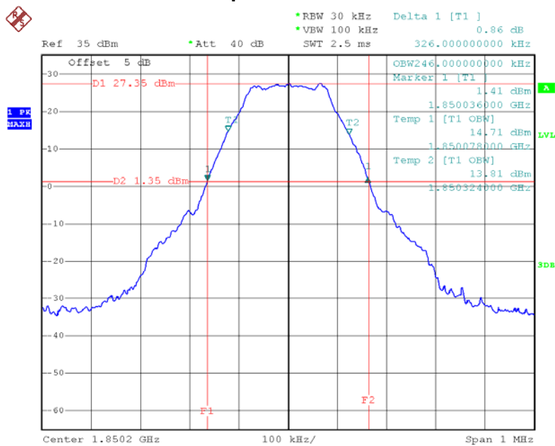
99% Occupied Bandwidth channel 512
