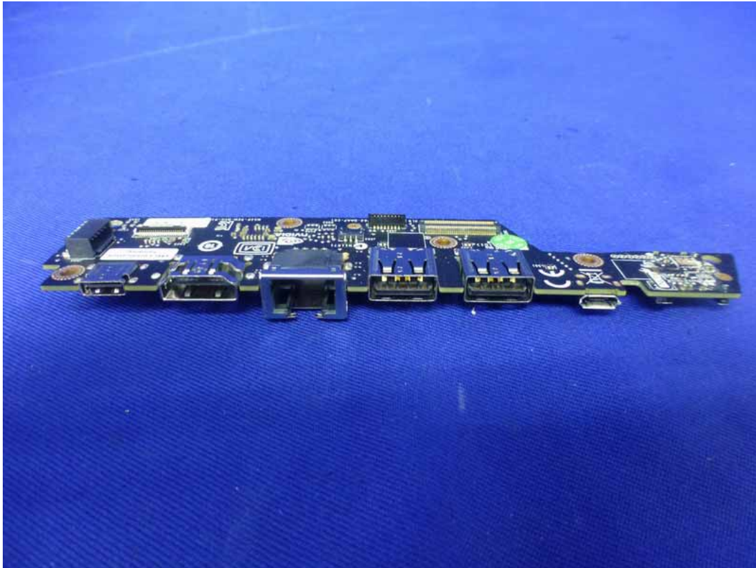
Figure 13 I/O Port of the Main Board
