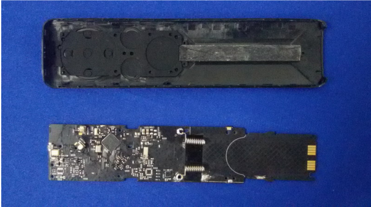
Figure 9 Inside of the EUT
