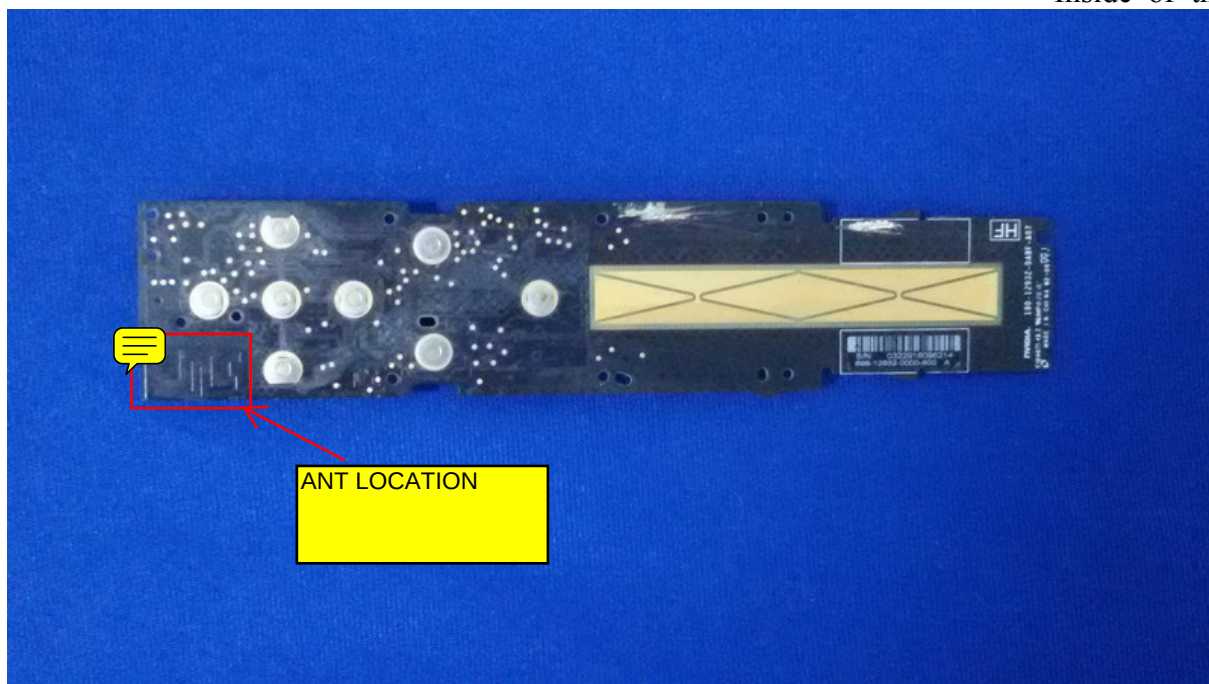
Figure 11 Inside of the EUT
