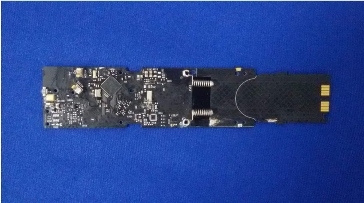
Figure 10 Inside of the EUT
