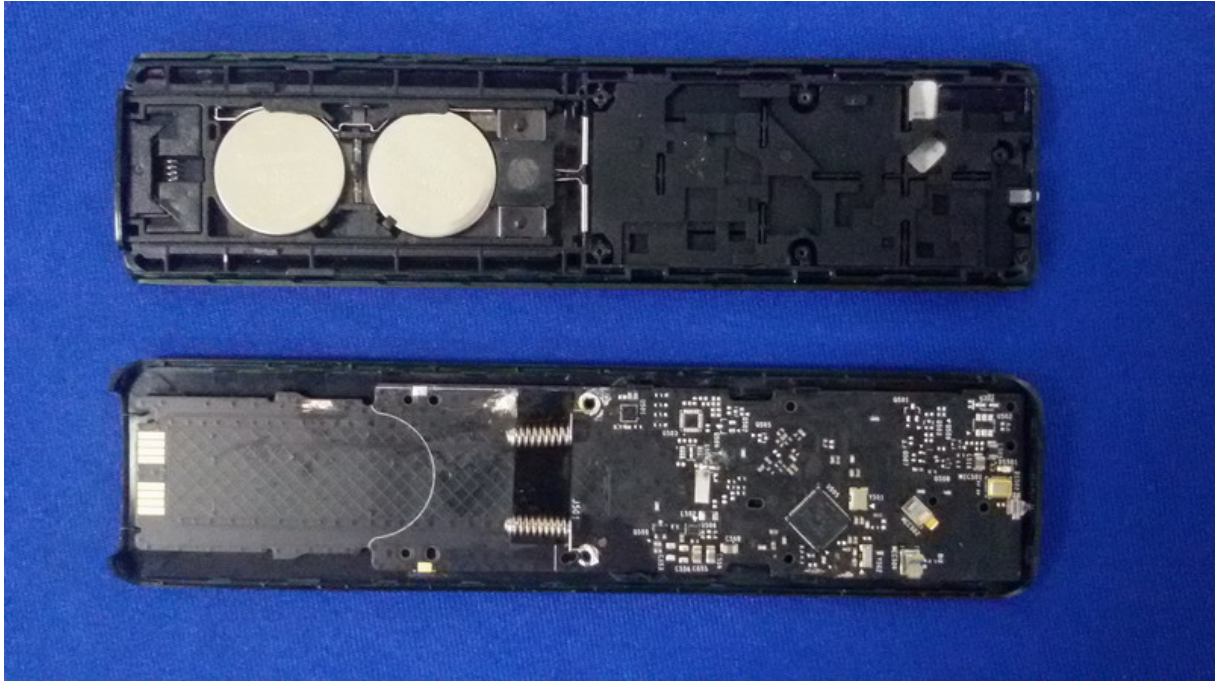
Figure 7 General Appearance of the EUT
