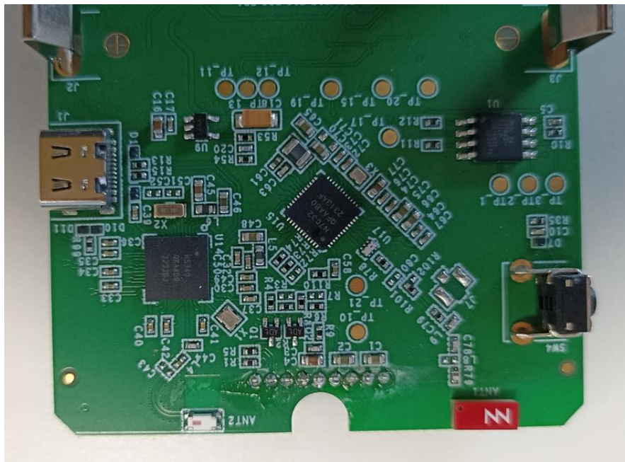
INTERNAL VIEW OF EUT – figure 4
