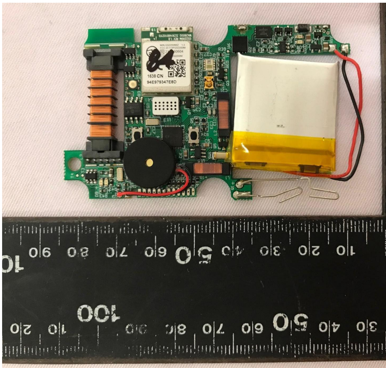
Main-Board PCB Component Side
