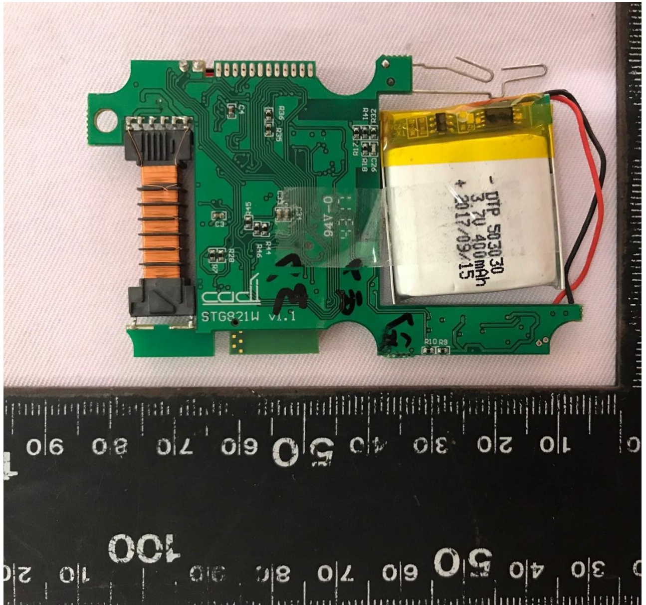
Main-Board PCB Trace Side
