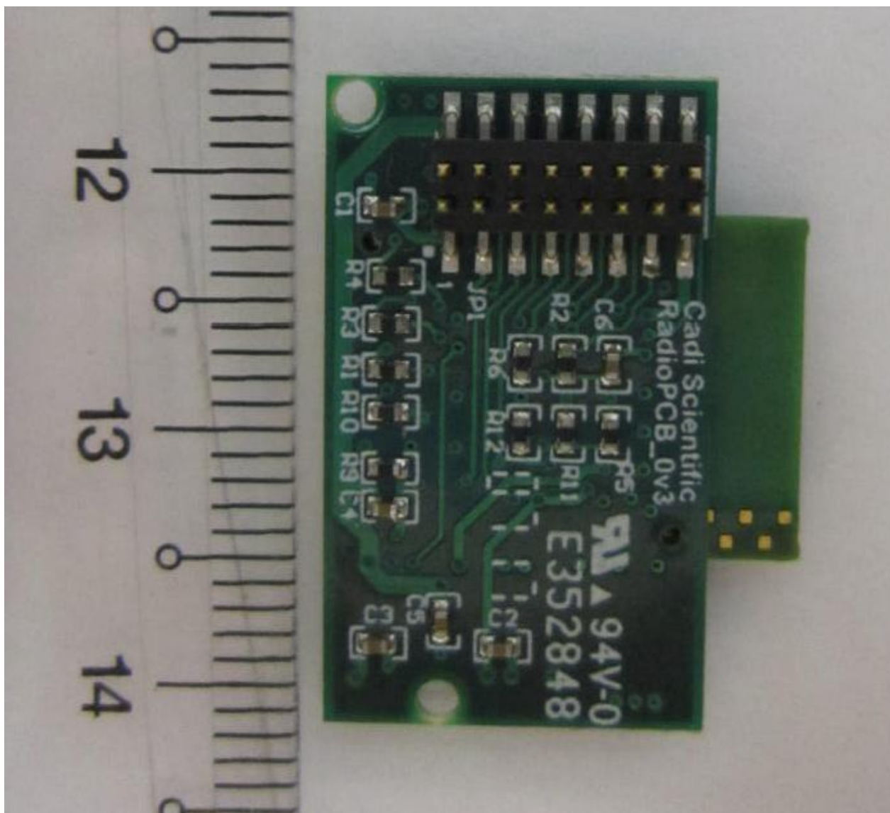
Module Board PCB Trace Side
