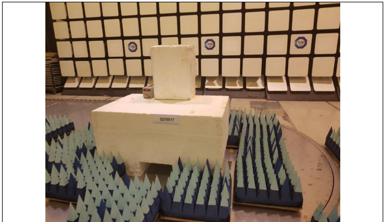
Band Edge Compliance (Radiated) Test Setup
