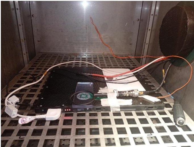
Photo of Field strength within the band 13.110-14.010MHz in Climatic Chamber
