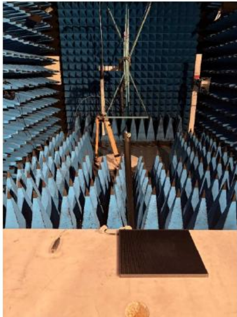
Test setup in anechoic chamber – Frequency <1GHz
