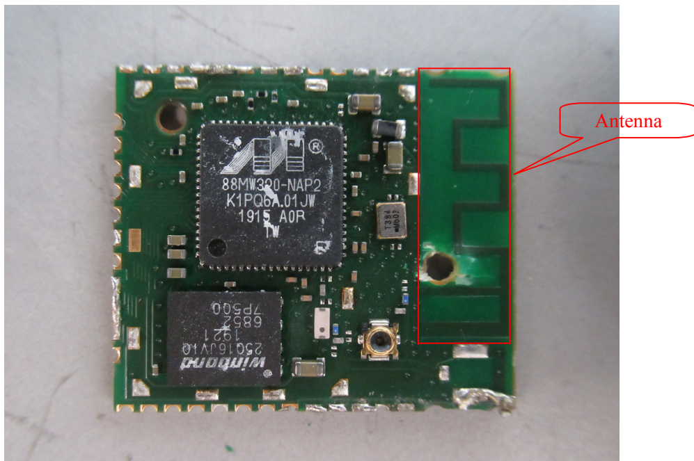
EUT – Top Chip View
