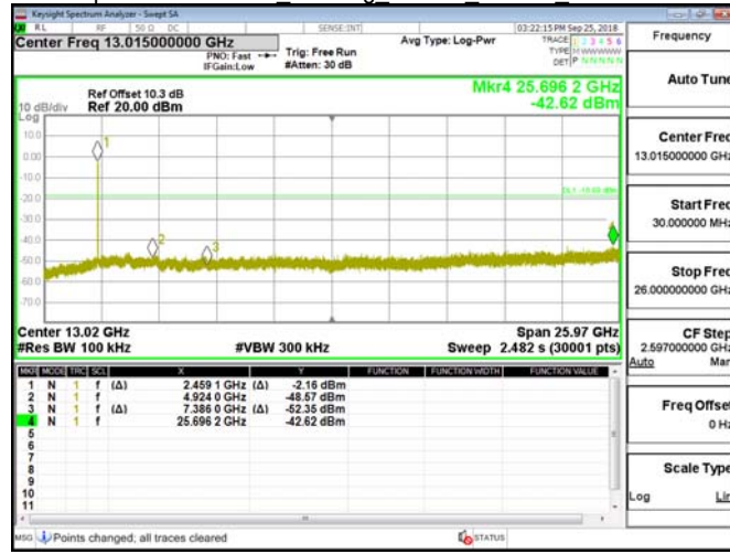
Spurious Emission 802.11g 20MHz Chain0 2462MHz
