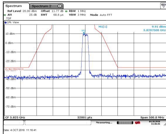
Figure 7.3.2-2: Radiated BE Upper – 802.11a
