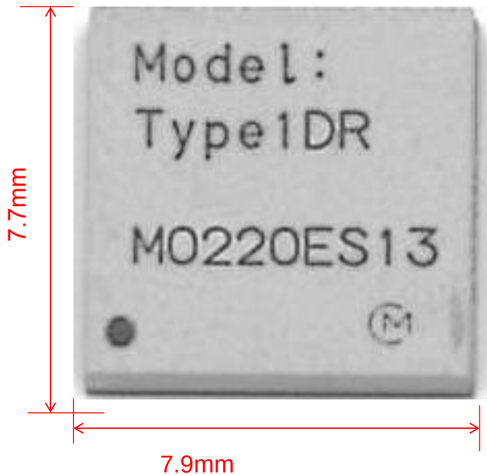
Module(Top --- Shielded)
