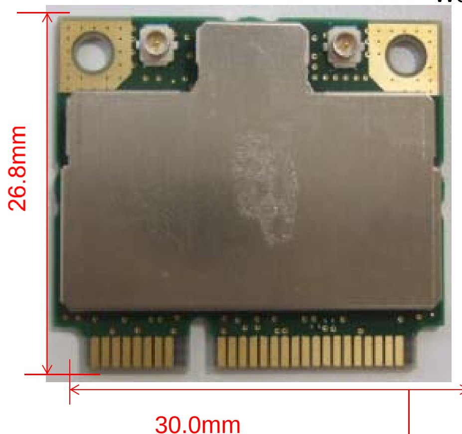
Module(Top --- Shielded)
