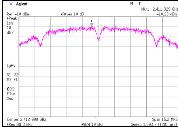
11b Antenna 1
