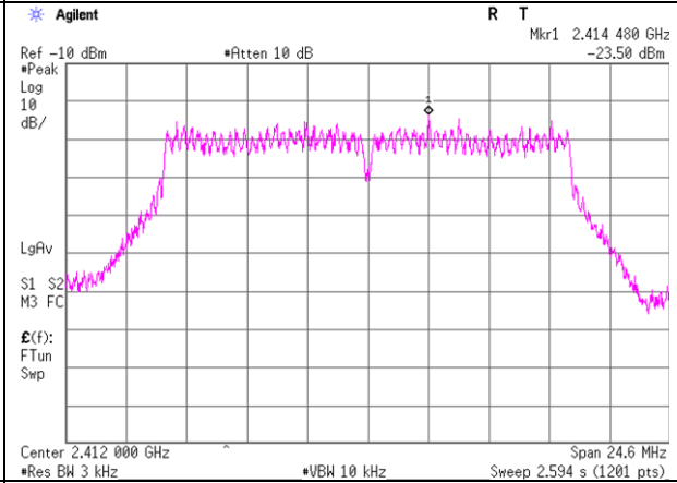
11g Antenna 1
