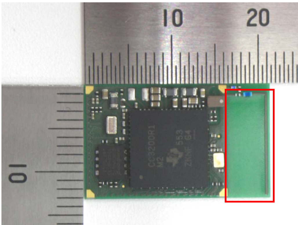
Antenna Location
