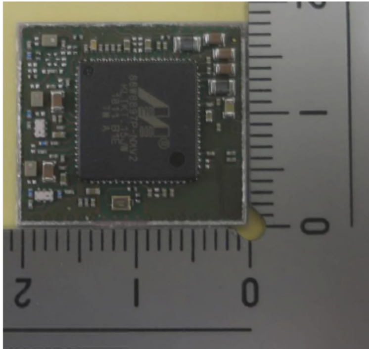
Internal View of EUT-2
