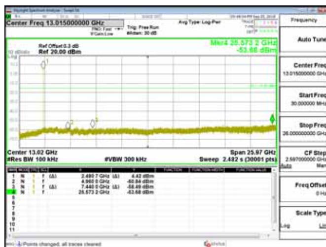
Spurious Emission_π/4DQPSK_2M_2480MHz
