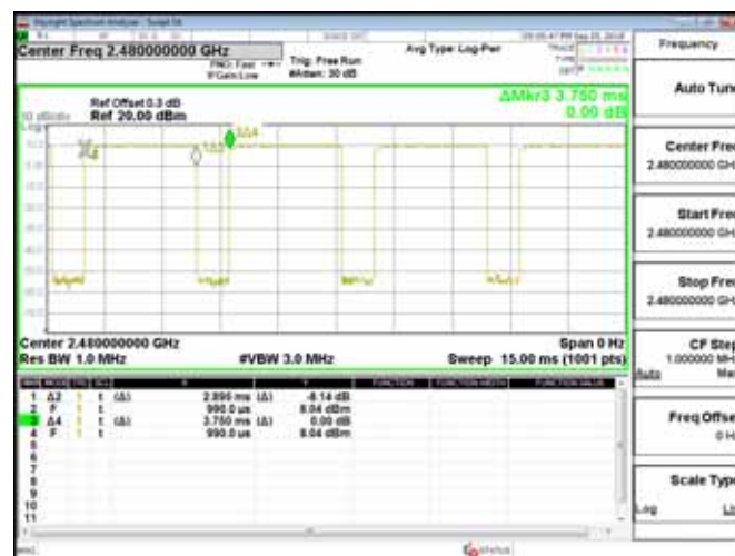
Dwell Time_π/4DQPSK_2M_DH5_2480MHz
