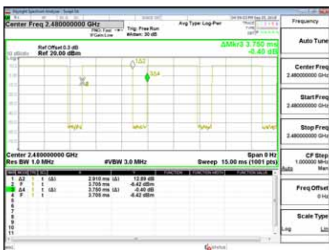
Dwell Time_GFSK_1M_DH5_2480MHz
