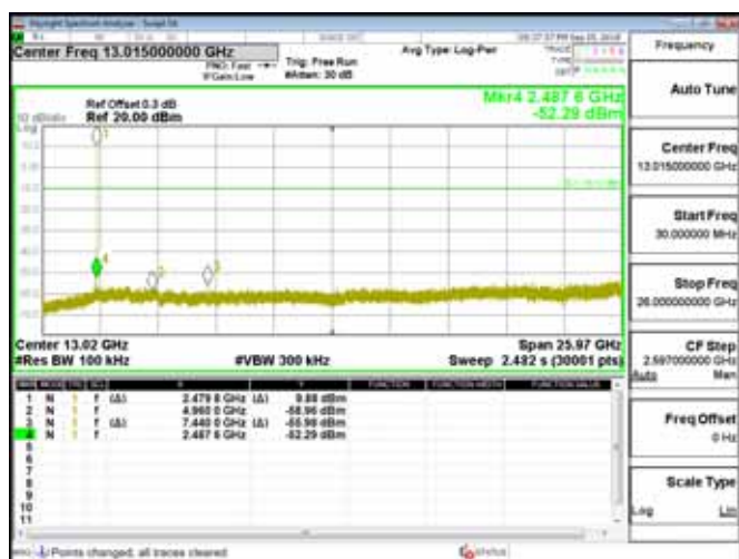
Spurious Emission_GFSK_1M_DH5_2480MHz
