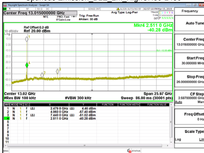
Spurious Emission BLE 2M HighCH39-2480
