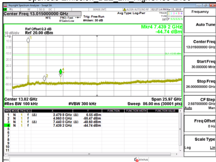
Spurious Emission BLE 1M HighCH39-2480
