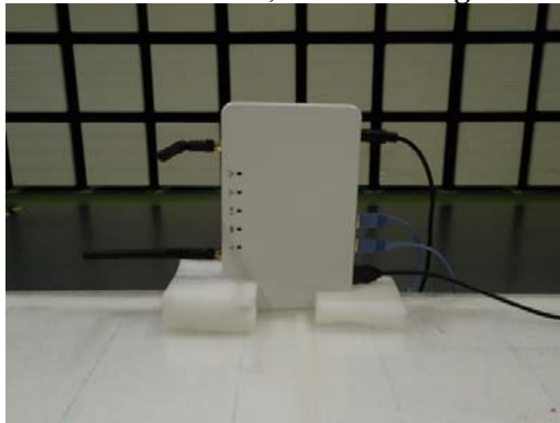
EUT Z-axis, ANT2 90 deg
