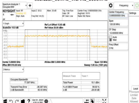
802.11ax_80MHz_WLAN1_5690MHz
