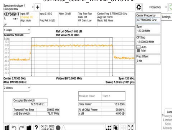
802.11ax_80MHz_WLAN2_5775MHz
