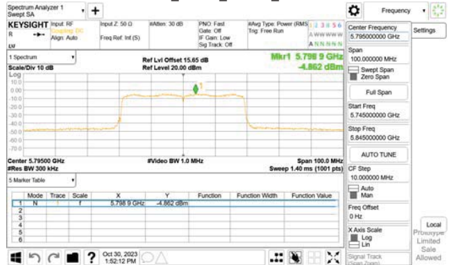
802.11ax_40MHz_WLAN2_5795MHz_RU242 62
