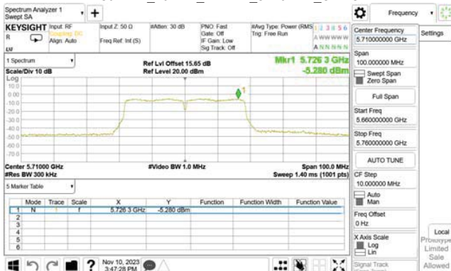
802.11n_40MHz_WLAN2_5710MHz_UNII 3
