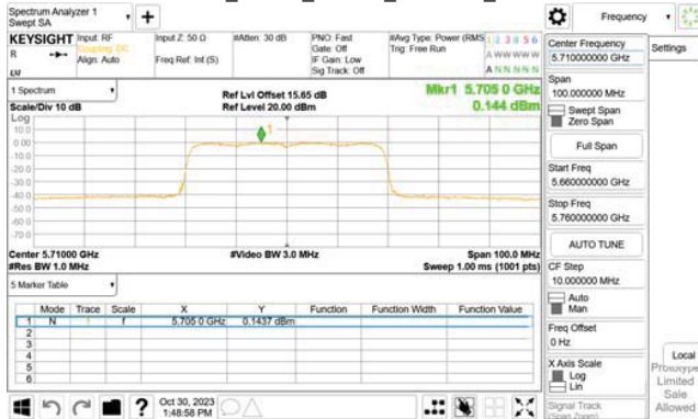
802.11ax_40MHz_WLAN2_5710MHz_UNII 3
