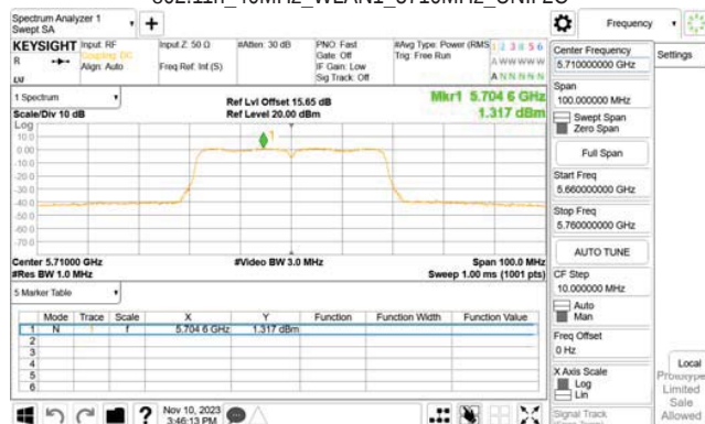
802.11n_40MHz_WLAN1_5710MHz_UNII 2C
