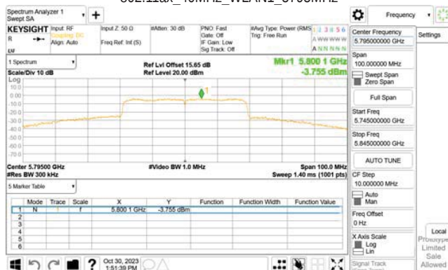
802.11ax_40MHz_WLAN1_5795MHz
