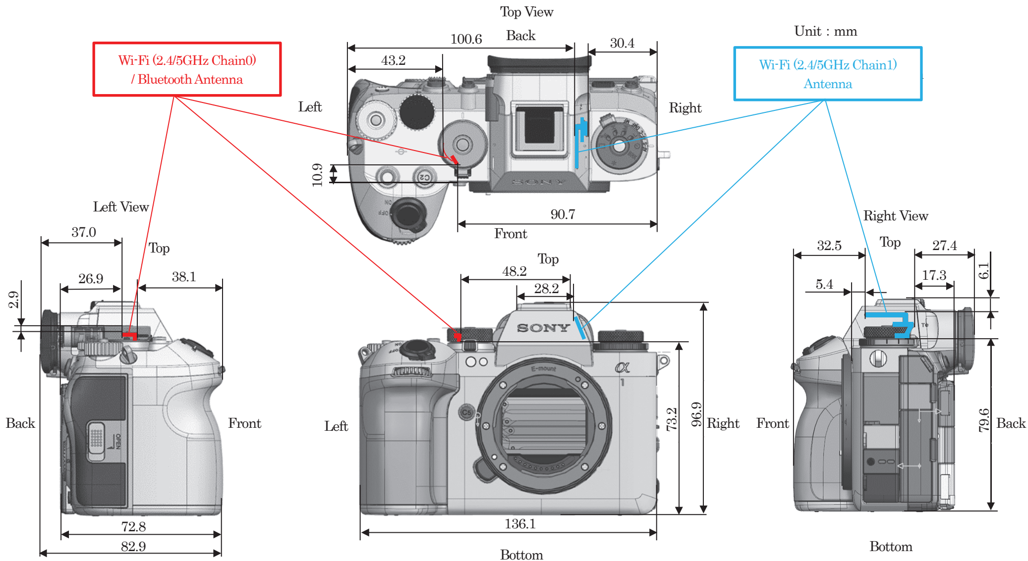
Figure D-7 Antenna Dimensions and Separation Distances
