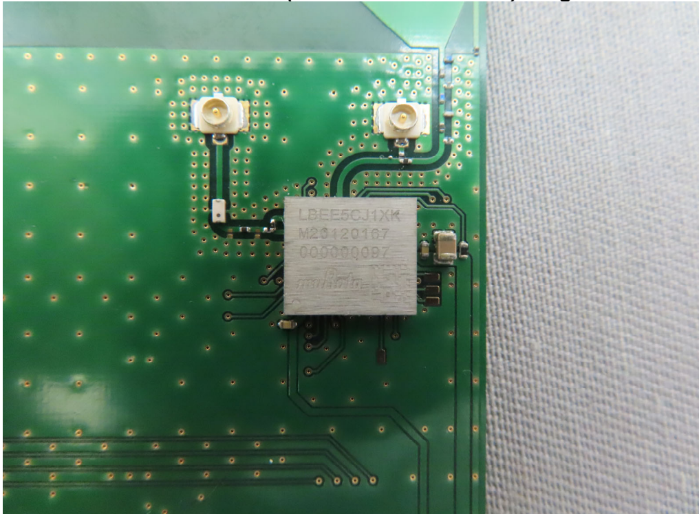
Front View of EUT-2 (Model: LBEE5CJ1XK) Diagram B
