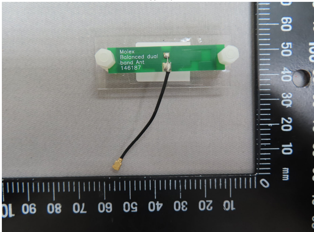
Antenna-2
